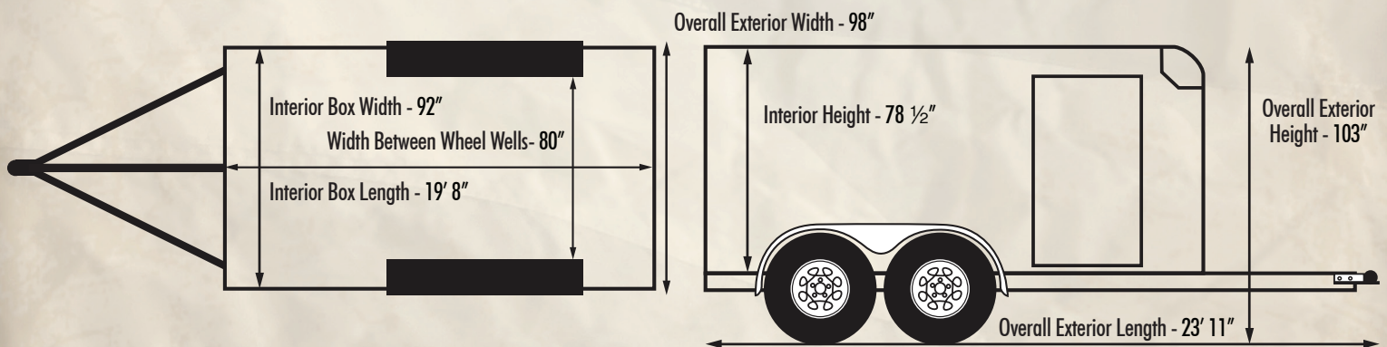
8' Wide Standard model CM820C-CT shown
