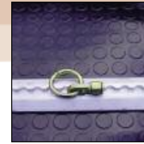
Rubber Coin Pattern Floor, Tapered Aircraft Track & Double Stud Tie-Down Ring
